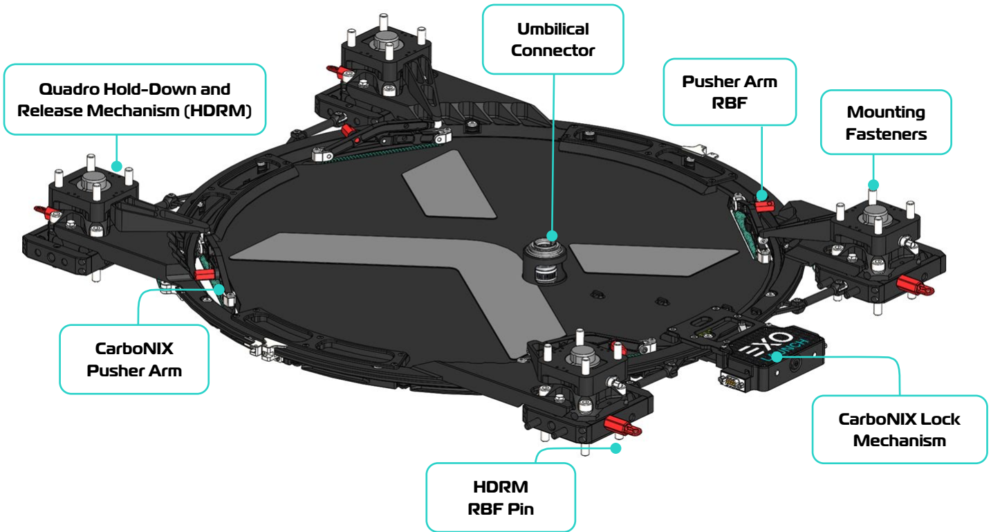
Figure 2: Quadro components overview.
