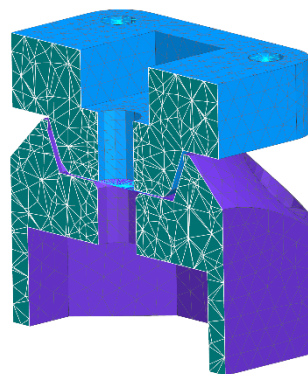
Figure 9: Quadro HDRM Finite Element Model
