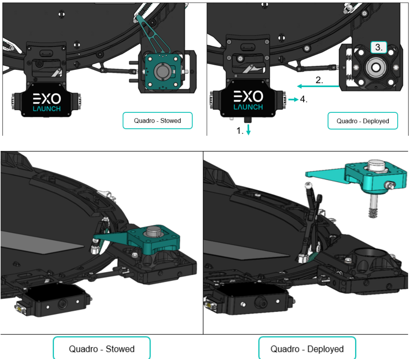
Figure 6: Quadro step-by-step deploy sequence.
