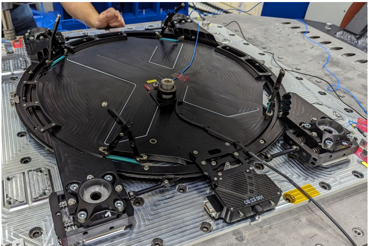
Figure 5: Quadro system under test.
