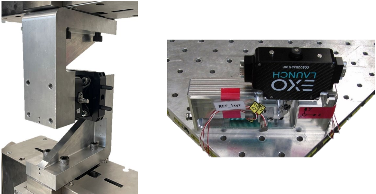
Figure 4: Quadro HDRM Strength Qualification (left) and Shock Qualification (right)
