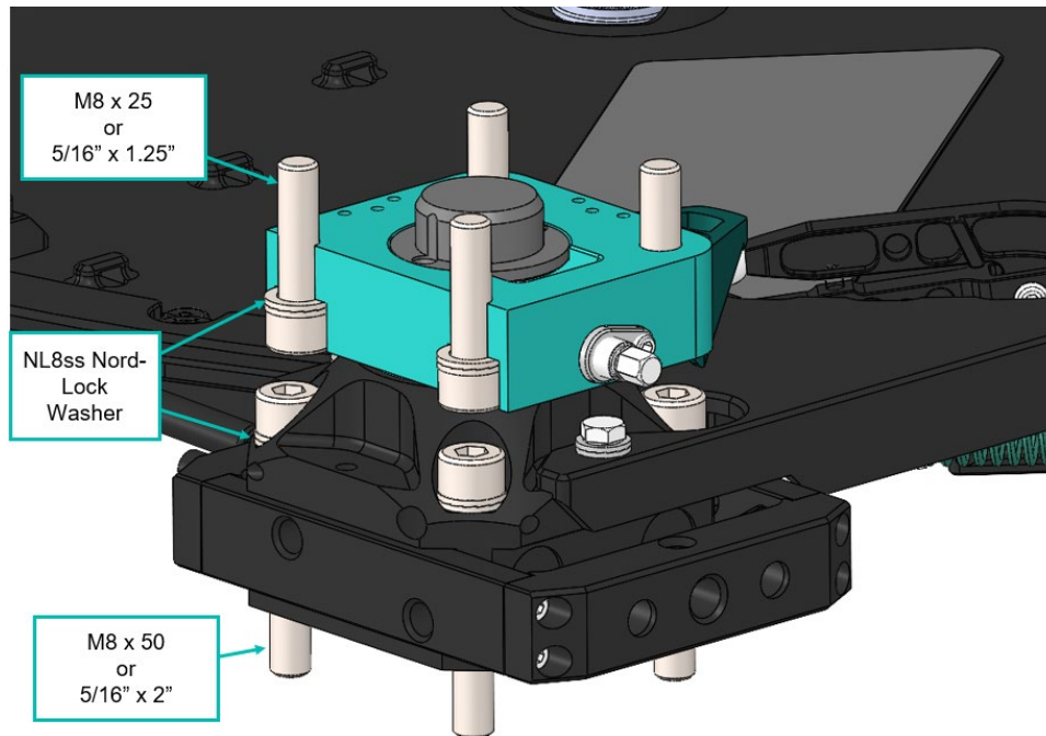
Figure 8: Quadro Mounting Configuration
