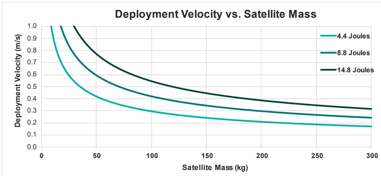
Figure 10: Quadro Separation Velocity
