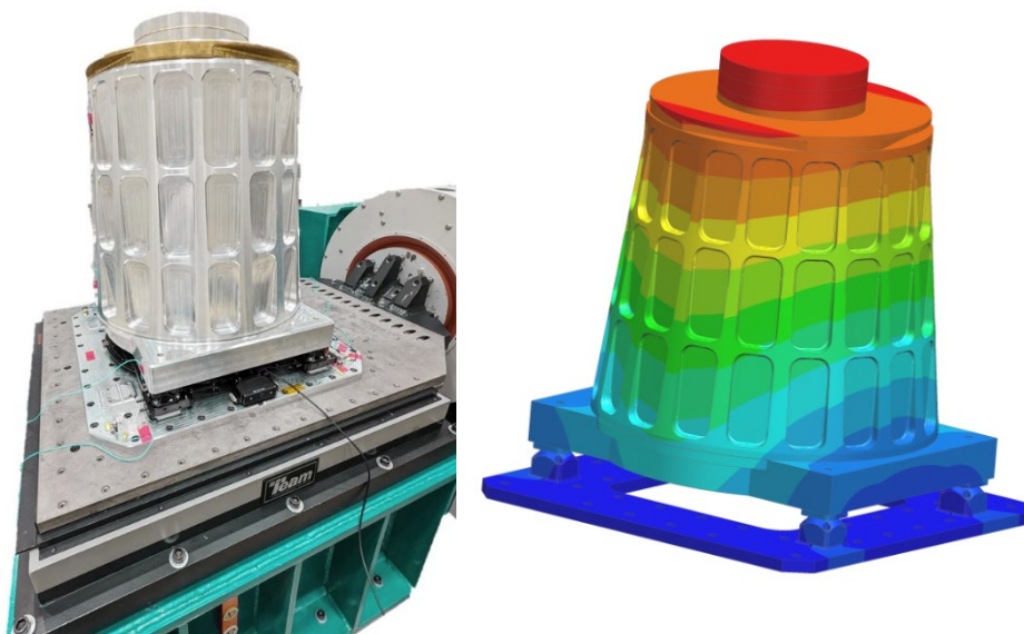
Figure 3: Quadro HDRM Vibration Qualification (left) and Correlation (right)
