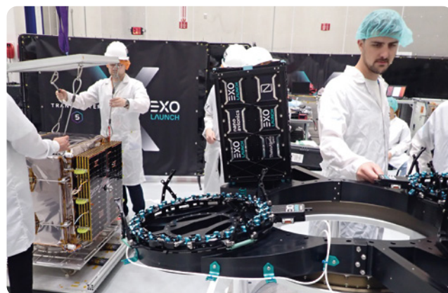
3 EXOport Multi-Satellite Adapter
